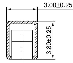
SEC:C-C
