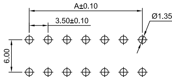
P.C.B LAYOUT TOLERANCE:±0.05
