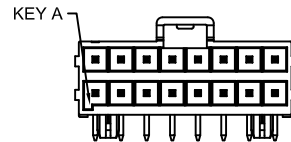
2x4P~2x12P KEY A
