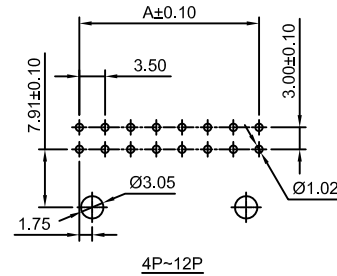
P.C.B LAYOUT TOLERANCE:±0.05
