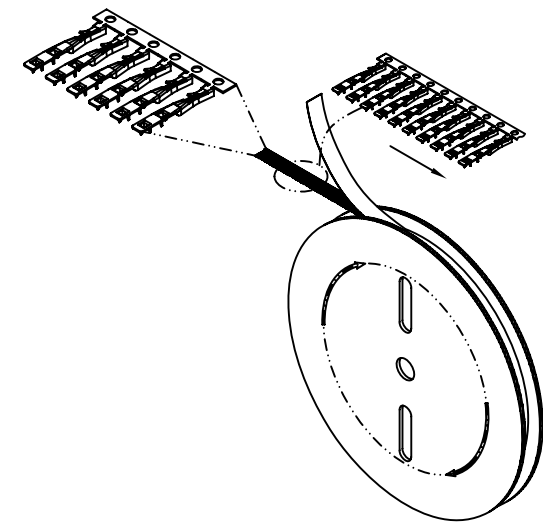
Winding Direction
