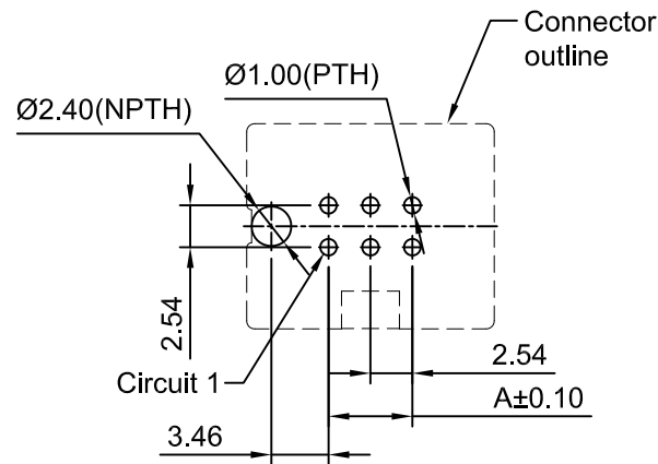
P.C.B LAOUT (TOP VIEW) TOLERANCE:±0.05
