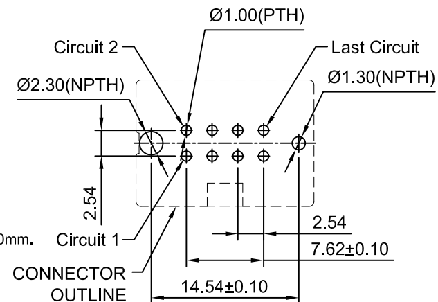
P.C.B LAYOUT(TOP VIEW) TOLERANCE:±0.05
