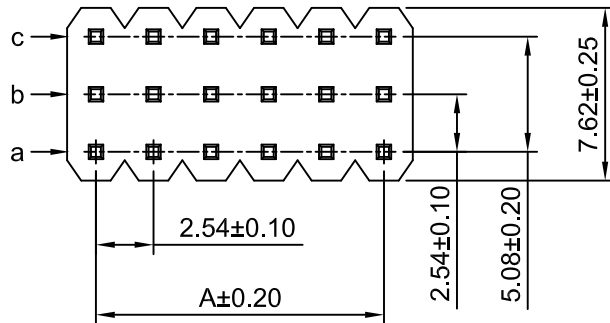
P.C.B LAYOUT TOLERANCE:±0.05
