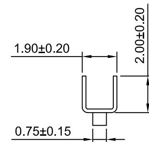
SEC:C-C
