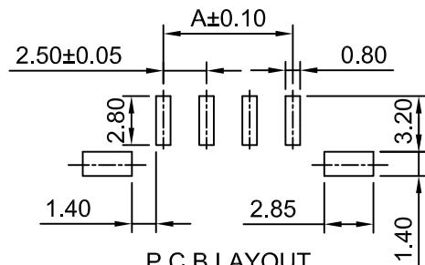
P.C.B LAYOUT TOLERANCE:±0.05
