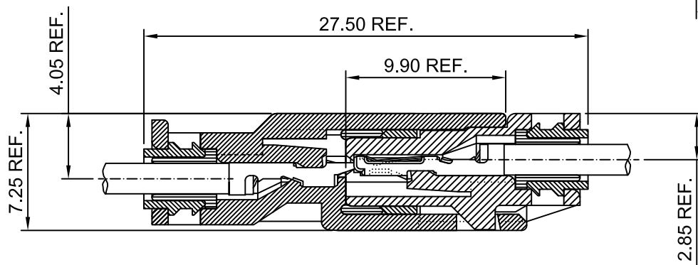
ASSEMBLY LAYOUT MATED WITH A2509HMC-2P
