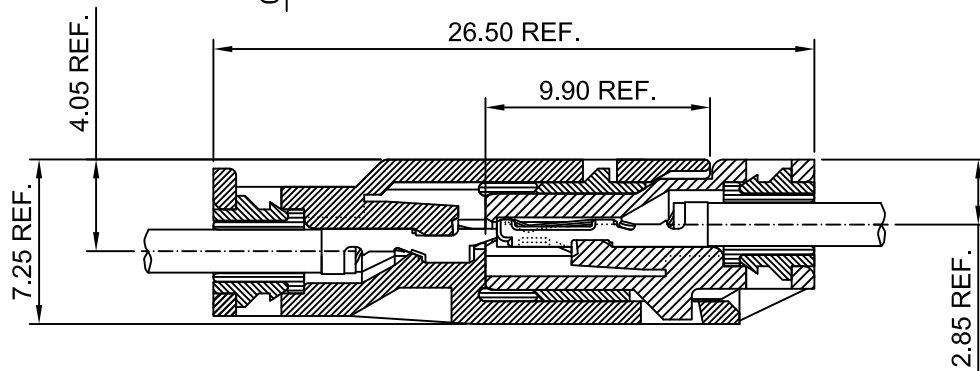
ASSEMBLY LAYOUT MATED WITH A2509HMC-4P
