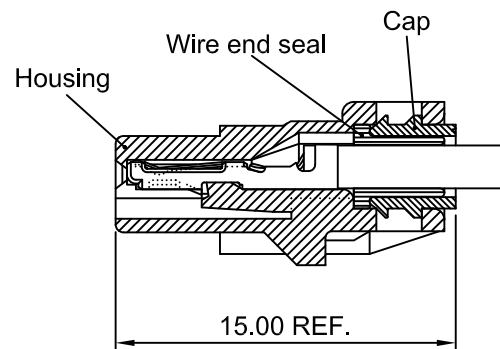
ASSEMBLY LAYOUT USED WITH A2509F-T-C
