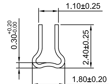
SEC:C-C
