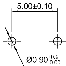
P.C.B LAYOUT TOLERANCE:±0.05
