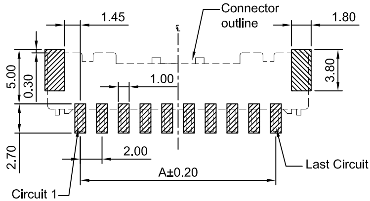
P.C.B LAYOUT (TOP VIEW) TOLERANCE:±0.05
