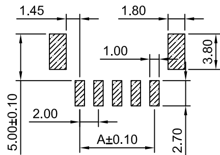
P.C.B LAYOUT TOLERANCE:±0.05
