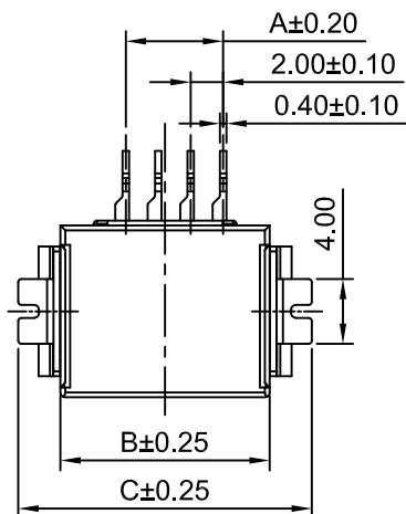
4P Type 1
