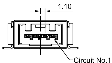
4P Type 1
