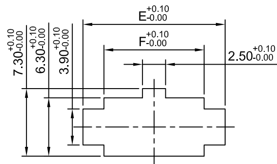
Panel Hole Layout Thickness:1.00~1.60mm
