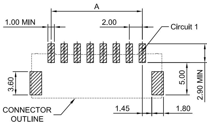
P.C.B LAYOUT(TOP VIEW) TOLERANCE:±0.05
