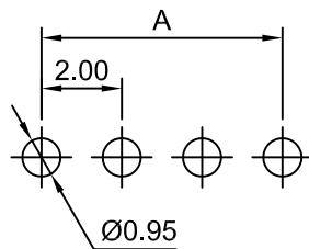
P.C.B LAYOUT TOLERANCE:±0.05
