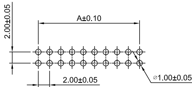
P.C.B LAYOUT (REFERENCE PCB T=1.20~1.60mm)
