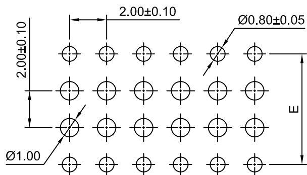
P C B LAYOUT
