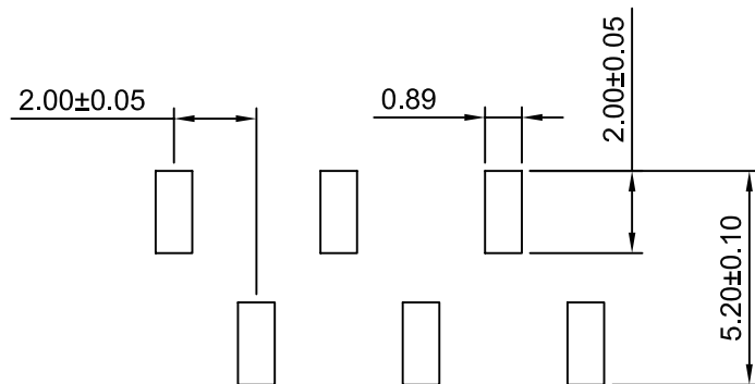
P C B LAYOUT
