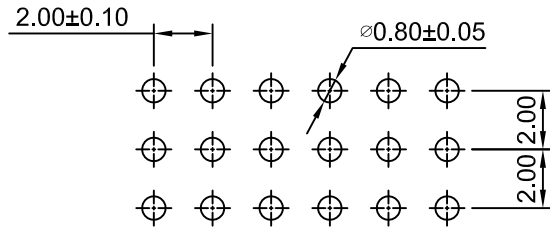
P C B LAYOUT
