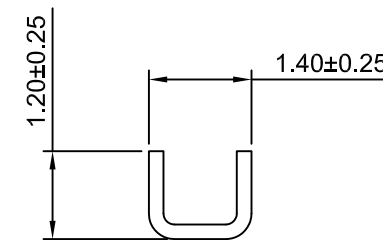
SEC:C-C
