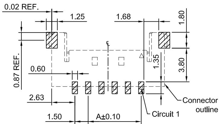
P.C.B LAYOUT (TOP VIEW) TOLERANCE:±0.05
