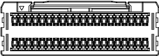
COMMON WITH ODD&EVEN CAVITY 2x10P~2x20P
