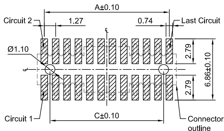
PCB LAYOUT (TOP VIEW) TOLERANCE:±0.05
