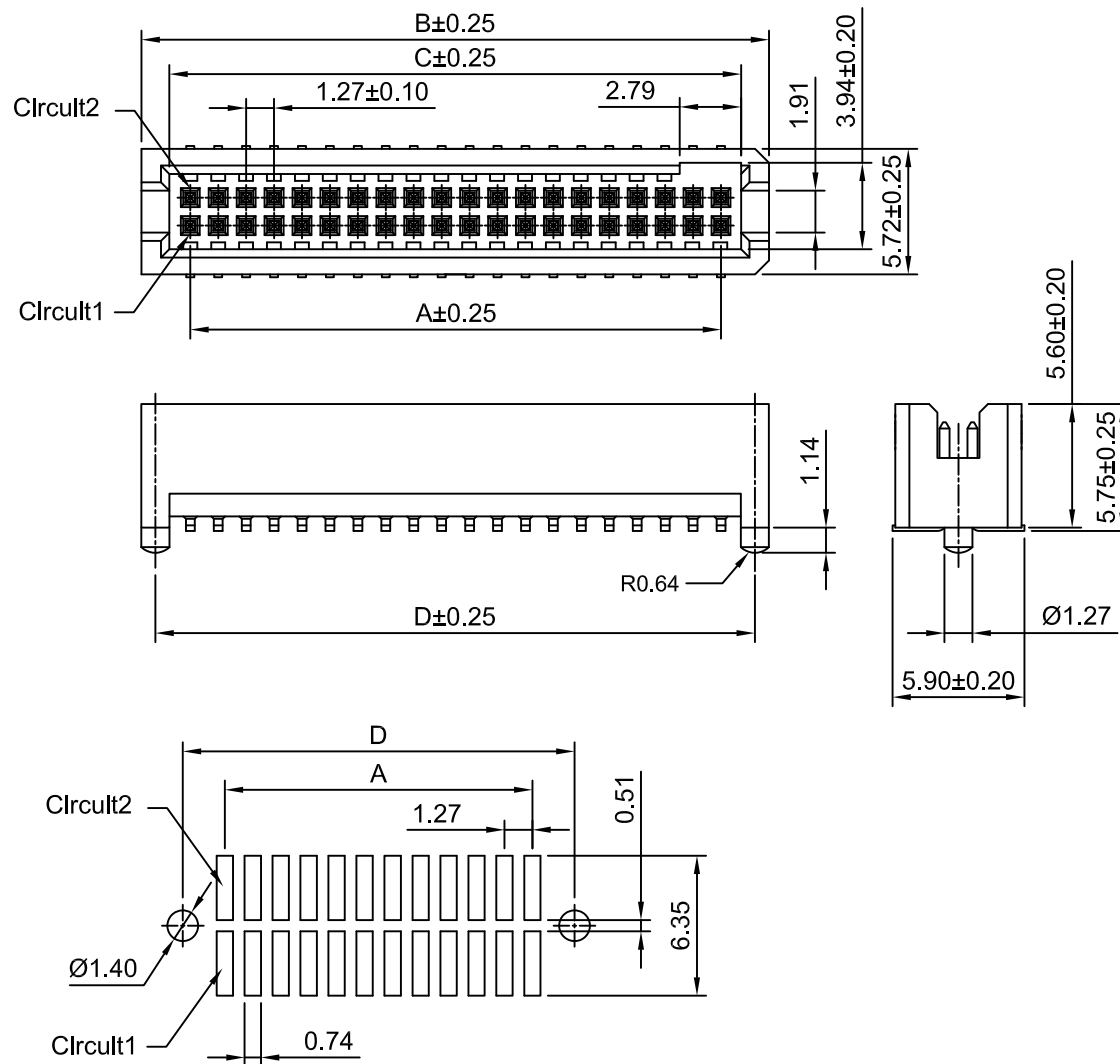
P.C.B LAYOUT (TOP VIEW) TOLERANCE: ±0.05
