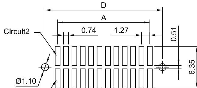
P.C.B LAYOUT(TOP VIEW) TOLERANCE:±0.05
