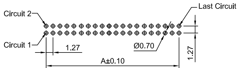
P.C.B LAYOUT TOLERANCE:±0.05
