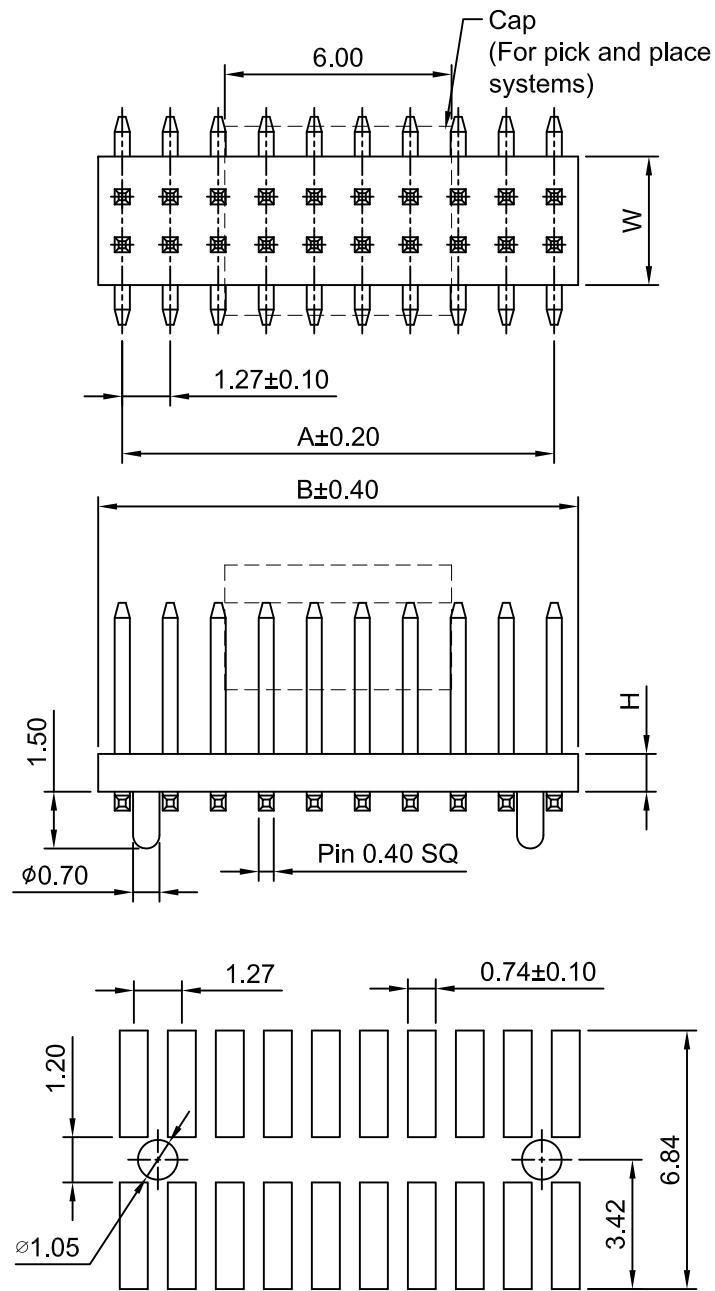
P.C.B LAYOUT TOLERANCE:±0.05
