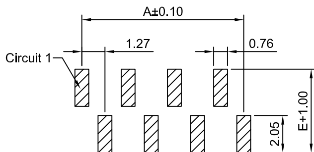
P.C.B LAYOUT TOLERANCE:±0.05
