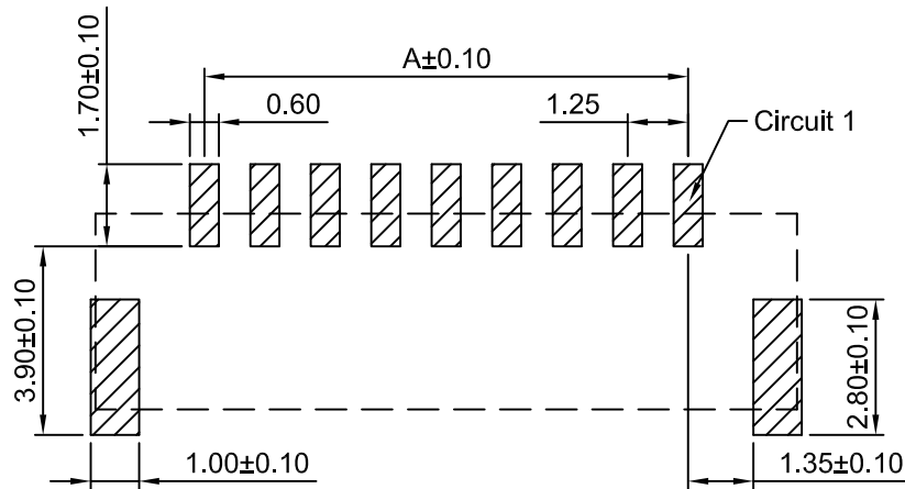
P.C.B LAYOUT TOLERANCE:±0.05
