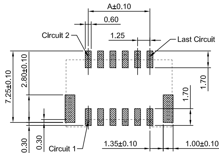
P.C.B LAYOUT(TOP VIEW ) TOLERANCE:±0.05
