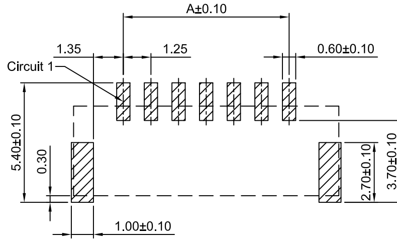
P.C.B LAYOUT TOLERANCE:±0.05
