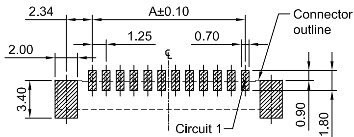
P.C.B LAYOUT (TOP VIEW) TOLERANCE:±0.05
