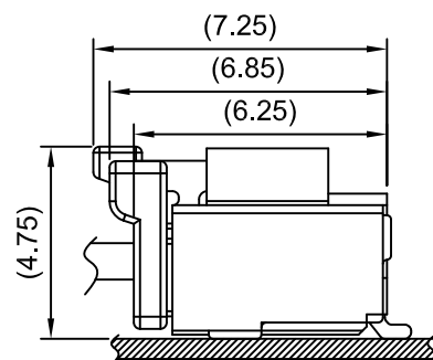
Mated Connectors
