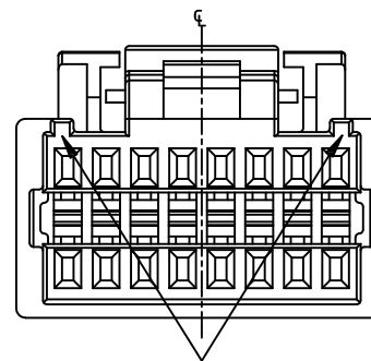
2x8P With Tow Guide Rib
