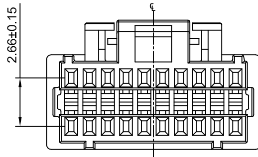
2x10P ~2x25P With Four Guide Rib
