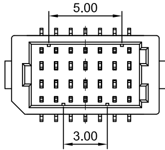
2x7P
