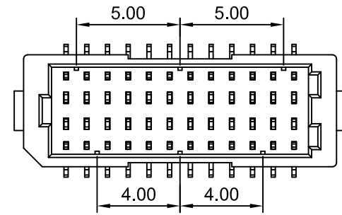
2x12P
