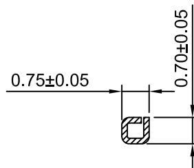
SEC:C-C
