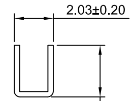
SEC:C-C
