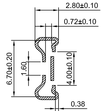
SEC:C-C
