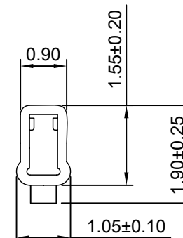
SEC:C-C
